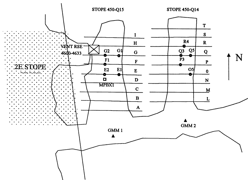
Figure 11: Plan view of the 4600 level showing the location of the instruments installed to monitor the Q14 and Q15 backs. The letters identify different cable bolt rings. In each ring a 'fanned' pattern of 8 cable bolts is placed. The vent raise plunges 75° to the north. Arrow is 5m long.
