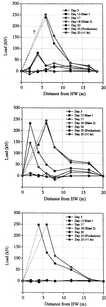
Figure 9: Load distribution along the SMART cables.
