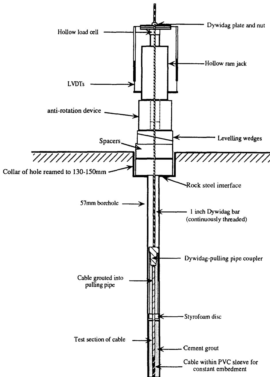
Fig. 7. Experimental set-up for in situ pull out test. It works equally well in the walls or floors of underground excavations.
