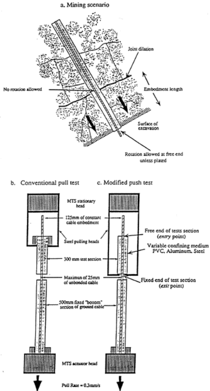
Figure 2. (a) Mining scenario and the laboratory pull test setups intended to simulate it: (b) the conventional pull test and (c) the modified push test used in this study.
