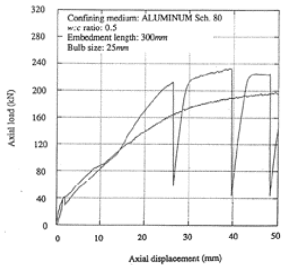
FIGURE 3d. Test GB4.
