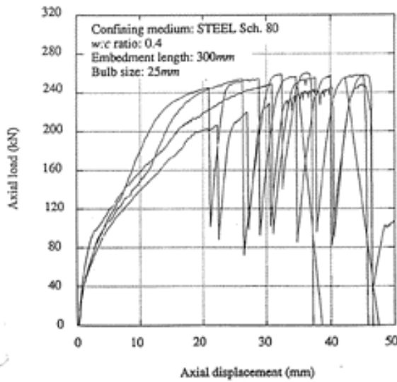
FIGURE 3b. Test GB2.
