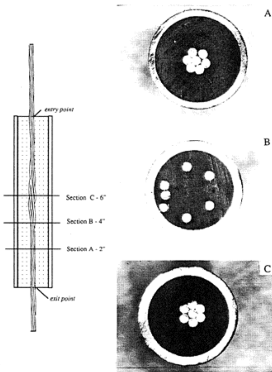
Figure 7 Sections through a 40mm specimen following failure
