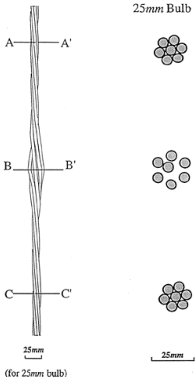
Figure 1. The Garford Bulb Anchor geometry
