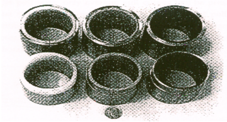
Figure 5 Pairs of deformable sleeves designed using FEM. They were inserted over the anchor (top) and the test (bottom) sections of the three different confining tubes.
