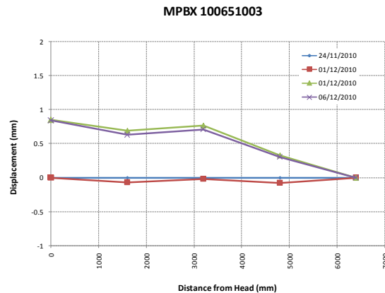
Figure 8: Displ. Distribution along length
