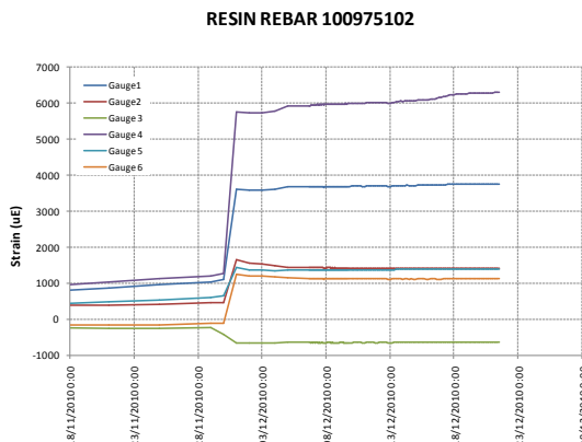
Figure 9: Strain displacement versus time
