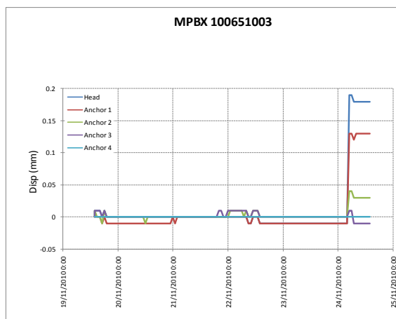
Figure 15: Displacement versus time
