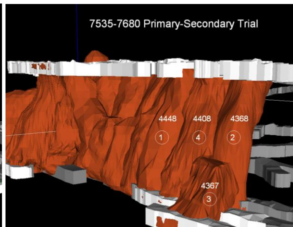
Figure 25: 4408 Secondary Stope Mined
