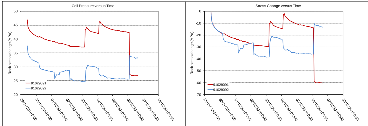
Figure 19: Time vs. longitudinal (091) and transverse (092) stress change record.
