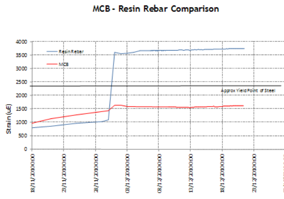
Figure 14: Comparison of Rebar & MCB
