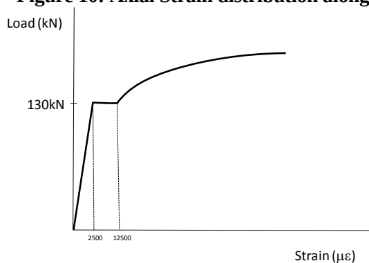
Figure 12: Load-Strain curve of rebar
