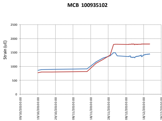
Figure 13: Strain displacement versus time MCB
