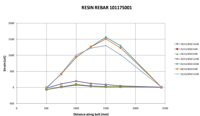
Figure 18: Strain along the length of rebar
