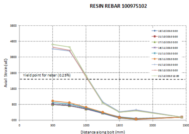
Figure 10: Axial Strain distribution along bolt
