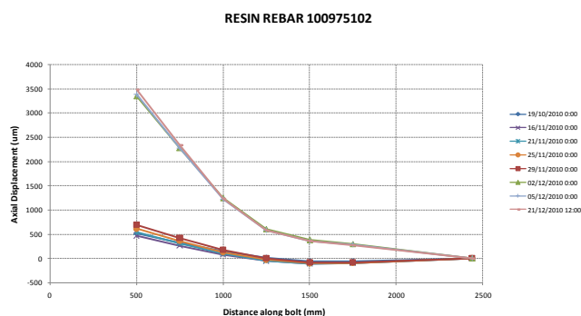
Figure 11: Stretch along the resin rebar
