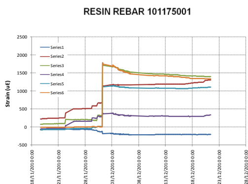
Figure 17: Strain versus time
