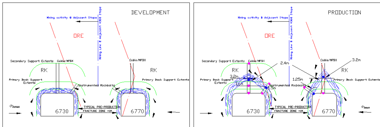
Figure 21: Induced fracture pattern around a development heading Creighton Deep Figure 22: Induced fracture pattern around development headings production & 1.7Mn event
