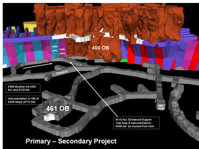
Figure 2: Mining geometry.
