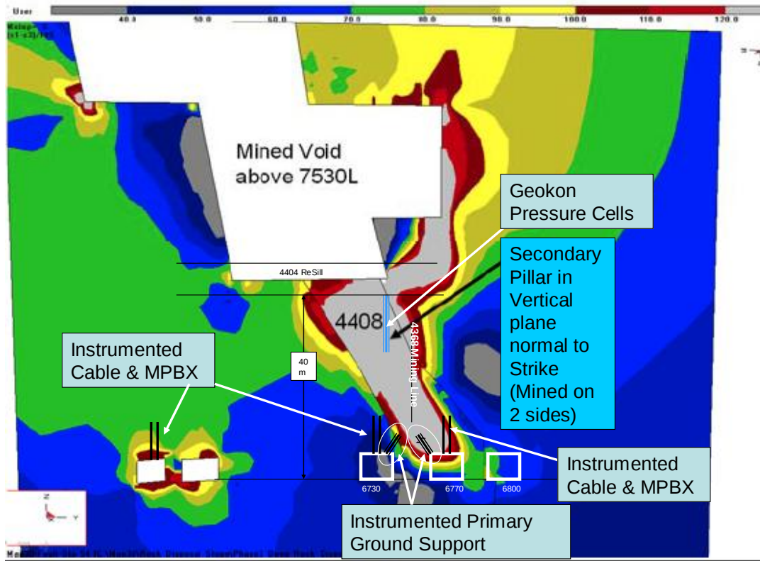
Figure 4 - Deviatoric Stress ( \sigma_1 - \sigma_3 ) at Diminishing Pillar showing instrumentation locations
