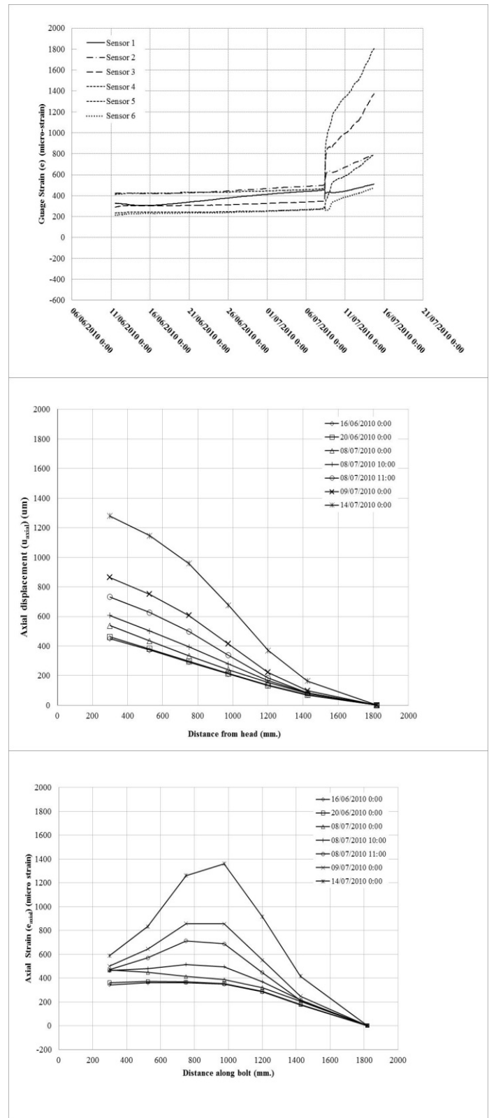
Fig.10: The response of a rock bolt #75 in case study 2 (upper) response of the 6 strain gauges with time (middle) Axial displacement versus length and (lower) bolt strain versus length (153µε/tonne).
