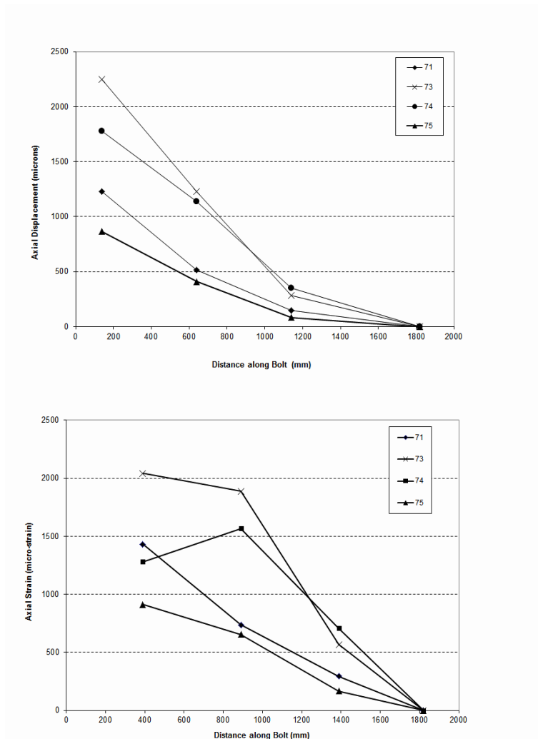
Figure 8: (Top) Axial stretch or displacement along the bolt length and (Bottom) strain distribution along the bolt length (153 \mu\epsilon /tonne)
